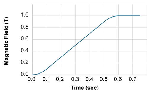
Figure 5: Excitation pattern of bending magnet.
