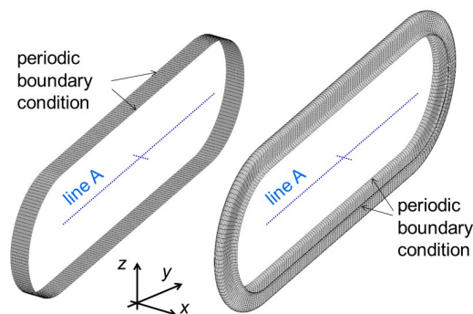
Figure 4: Numerical models of beam duct (unit period), flat structure (left) and bellows structure (right).
