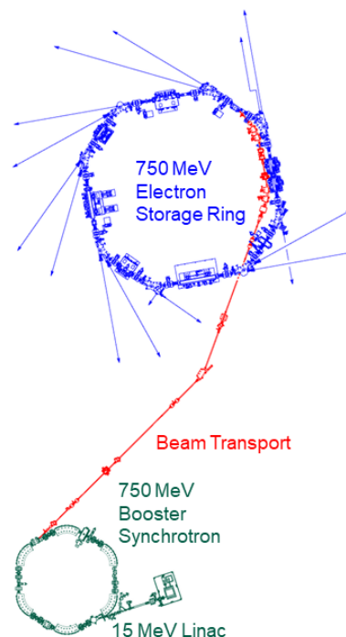
Figure 1: Accelerator layout of UVSOR.
