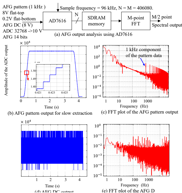
Figure 6: AFG output measurement and analysis.
