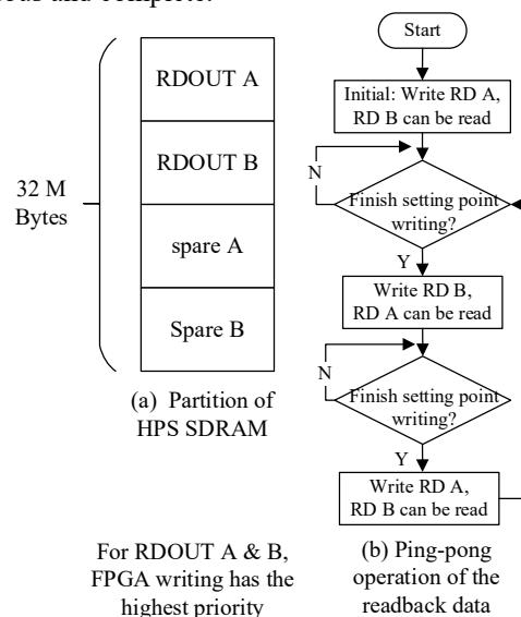
Figure 3: SDRAM partition and logic.
