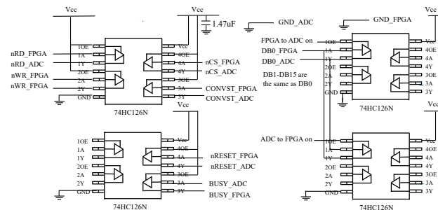
Figure 5: Schematic of the interface board.
