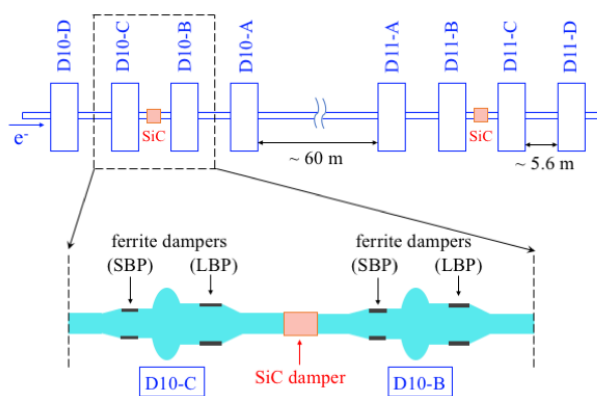
Figure 4: Layout of ferrite HOM dampers in the SCC with additional SiC dampers between the cavities.
