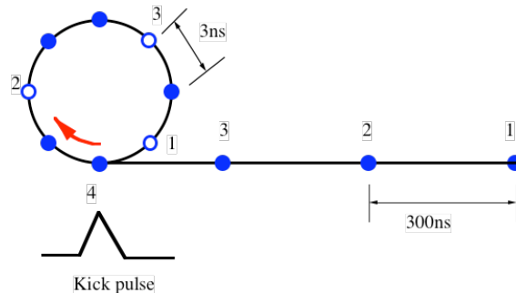
図1 Beam extraction from DR to Linac
