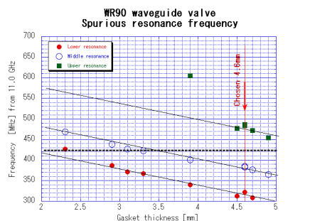
Fig. 6: Spurious resonance thickness frequency vs gasket thickness.
