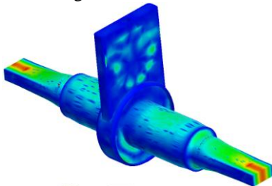
Fig. 5: Spurious resonance example.
