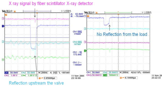
Fig. 9: Waveforms of breakdown events at the valve.
