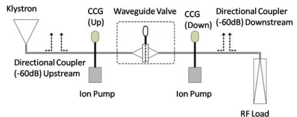
Fig. 7: High power test setup.
