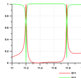
Fig. 3: S-parameters calculated by HFSS.
