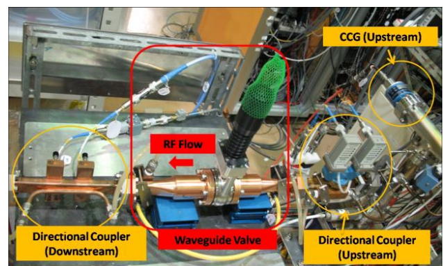
Fig. 8: The waveguide valve under test at KT-1, 50MW X-band station of KEK.
