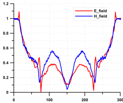
Fig. 4: E- and H-field along the axis.
