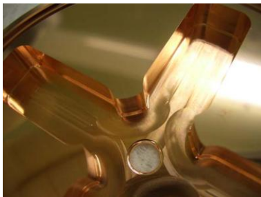
Figure 3: Detailed shape near iris of TD18 structure.
