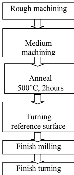
Figure 4: Machining flow chart of TD18 structure.
