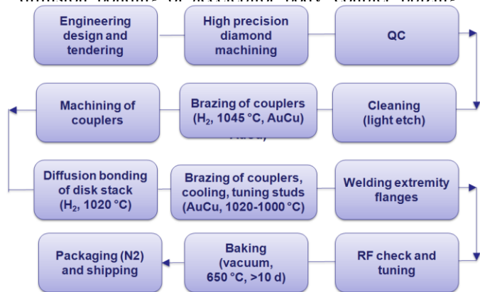
Figure 1: Manufacture flow chart.
