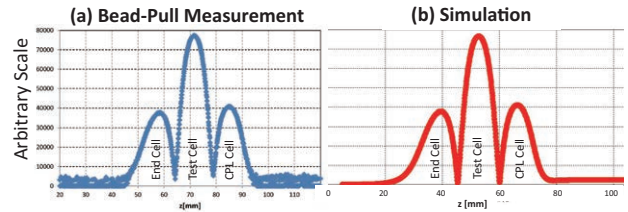
Figure 9: Comparison of the electric-field strength between the bead-pull measurement and simulation. CPL means coupling.
