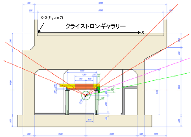
Figure8: A section view of the KEKB Injector Linac with the shielding structure for the positron target in the tunnel. The orange shield plates already exist and these will be reinforced by additional shields (indicated by yellow and green) for the reduction of radiation outside the Linac building.
