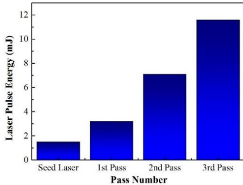
Figure 6: Laser pulse energy of the Peltier cooling multi-pass amplifier under 3.3 kW pump laser.
