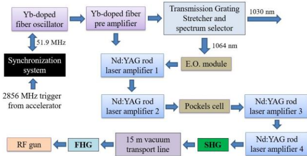
Figure 1: Layout of the Nd hybrid laser system for SuperKEKB Phase II commissioning.
