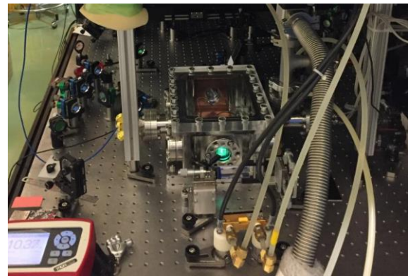
Figure 5: Experiment setup of Peltier cooling 3 pass multi-pass amplifier stage.
