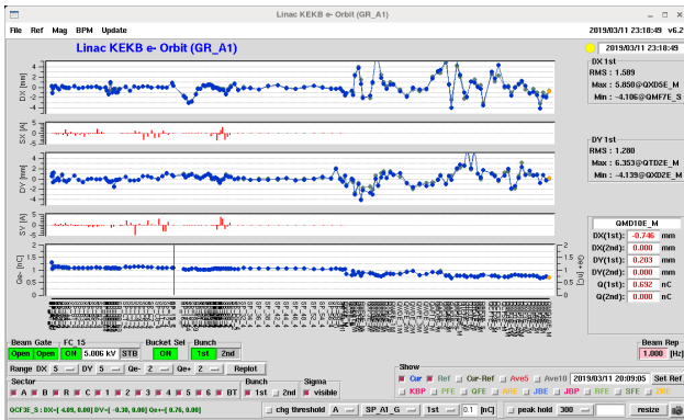
Figure 4: Electron orbit in phase III commissioning HER injection.
