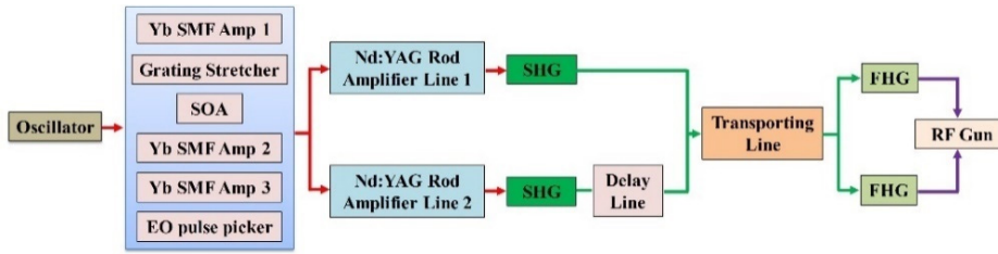
Figure 1: The layout of current Yb/Nd hybrid laser system for SuperKEKB phase III commissioning.
