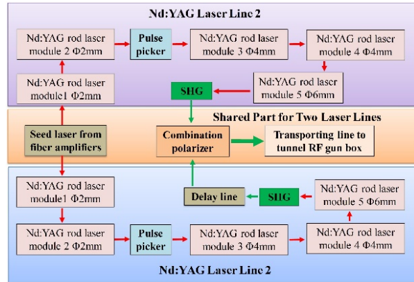
Figure 2: Configuration of the Nd:YAG rod laser amplification part of the current laser system.
