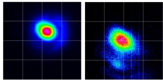
Figure 3: UV laser beam profiles of line 1 and line 2 at the position of virtual photocathode.
