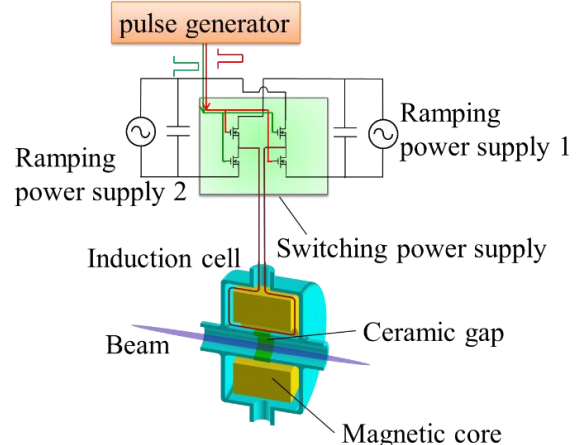
Figure 1: New acceleration control system for induction synchrotrons.
