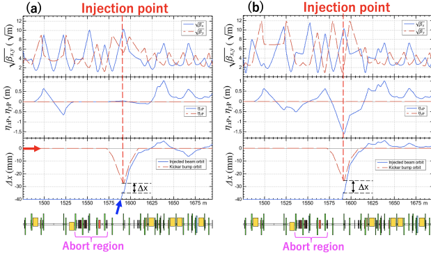
Figure 1: Optics and orbit plots for (a) BI and (b) SI. The top and middle plots show the beta and dispersion functions (blue: horizontal, red: vertical). The bottom plot shows the horizontal orbit: red and blue lines show the stored-beam kicker bump orbit and the injected beam orbit, respectively. The \Delta x shows the horizontal distance between stored and injected beam at the injection point.
