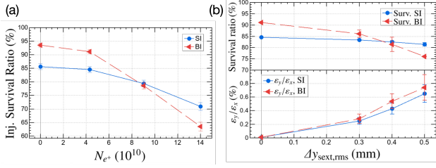
Figure 5: (a): The simulated dependence of the injection survival ratio on the bunch population of positrons, obtained by tracking with 1000 particles after 8000 turns from injection. The intensity N_{e^+} = 4.3 \times 10^{10} corresponds to the highest luminosity record 5.24 \times 10^{34}/\text{cm}^2\text{s} . (b): The simulated dependence of the survival ratio (upper) and the vertical emittance (lower) by random vertical misalignments for all sextupoles ( \Delta y_{\text{sext}} ) in the HER, with N_{e^+} = 4.3 \times 10^{10} .
