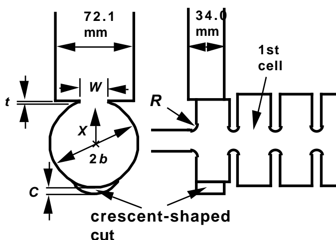
Fig. 1. Cross-sectional view of the coupler cavity ( R=7\text{mm} and t=2\text{mm} ).
