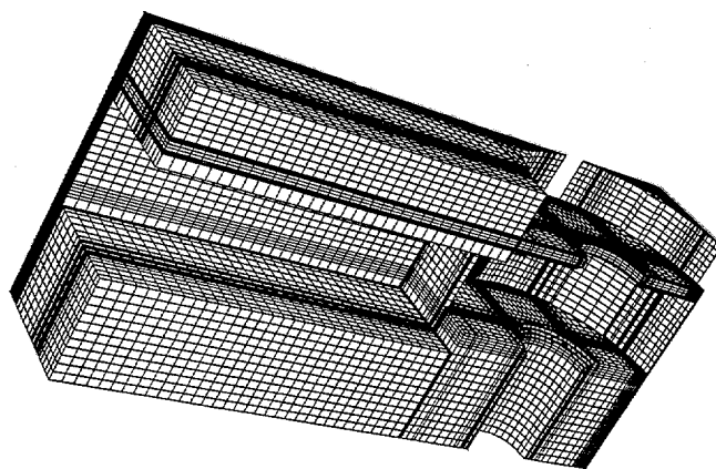
Fig. 2. MAFIA geometry for the Kyhl method simulation.
