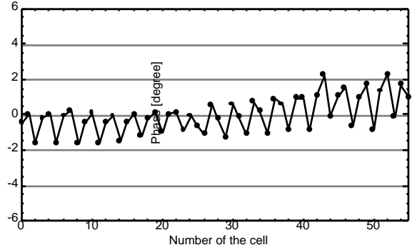
Fig. 8. Phase distribution for the accelerating structure after electron-beam welding of the couplers.
