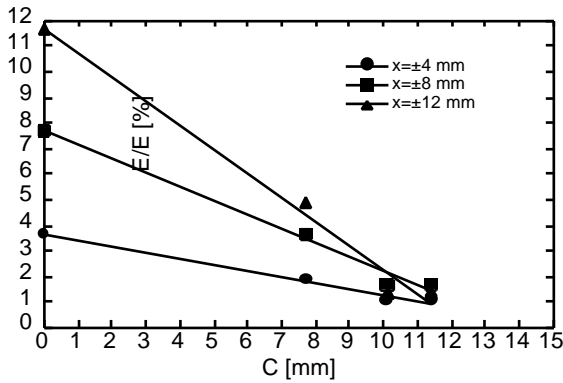
Fig. 6. E/E as a function of C .
