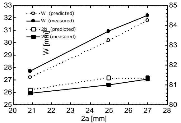
Fig. 5. Comparison between the predicted and measured values of W and 2b .
