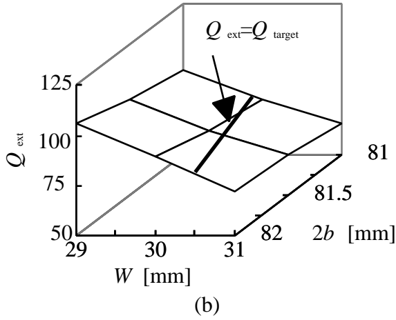
Fig. 3. (a) f_{res}(W, 2b) and (b) Q_{ext}(W, 2b) .
