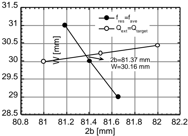
Fig. 4. Lines of f_{res} = f_{ave} and Q_{ext} = Q_{target} . The values at the cross point gives the designed values of W and 2b .
