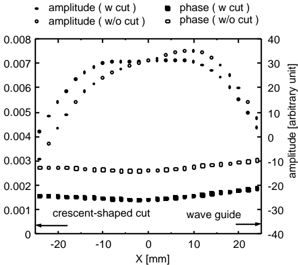
Fig. 7. Effect of the correction of an electromagnetic-field asymmetry by a crescent-shaped cut.
