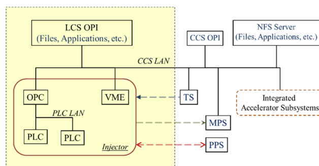
Figure 7: Integrated control system (Phase 3).
