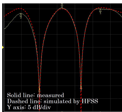
Figure 12: Transmission characteristics of output structure (solid-measured data, dashed- by simulation).
