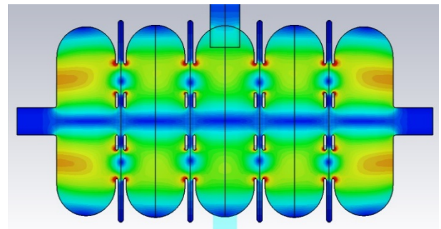
Figure 6: Electric field (abs).
