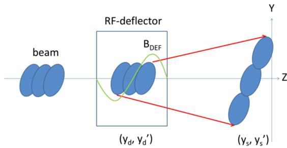
Figure 2: RF-Deflector.
