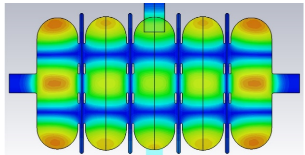
Figure 7: Magnetic field (abs).
