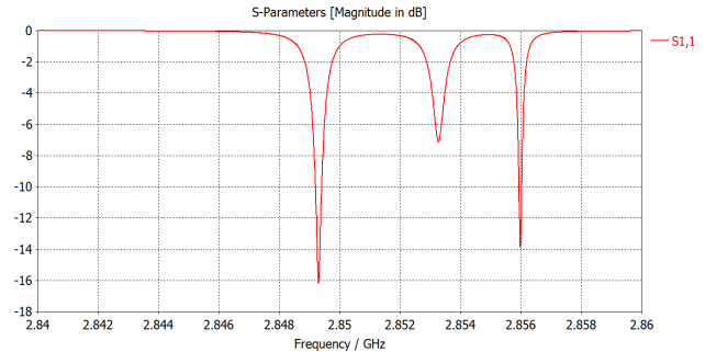
Figure 5: S-Parameter.
