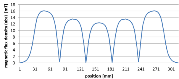
Figure 8: Plot of magnetic field (abs).
