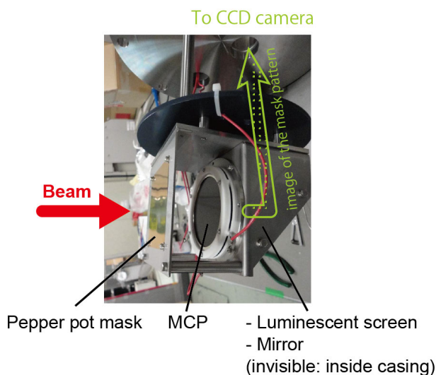
Figure 2: Photograph of the pepper pot emittance monitor. It consists of a pepper pot mask, a multichannel plate (MCP), a luminescent screen, a mirror and a CCD camera.
