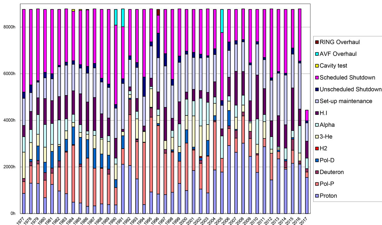
Figure 1: Operational statistics of the RCNP cyclotrons until the middle of 2017.
