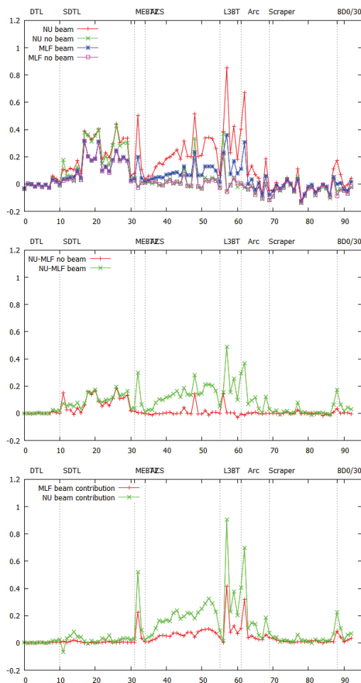
Figure 8: (Top) Typical “BLM display” plot for various pulse. (Middle) Difference between NU and MLF pulse mode. (Bottom) Beam contribution on BLMP signal.
