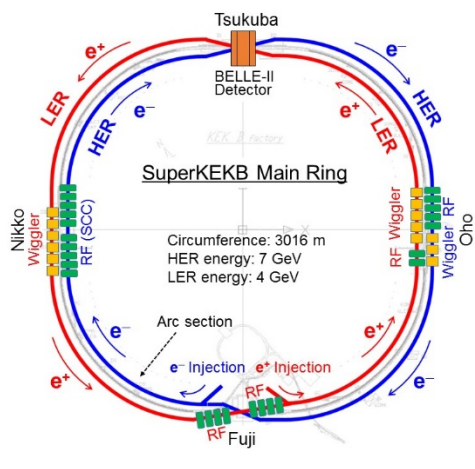
Figure 1: Layout of the SuperKEKB main ring.
