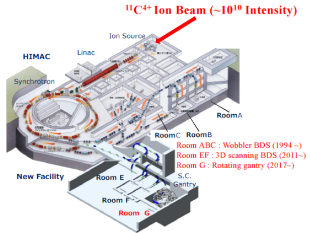
Figure 1: Layout of HIMAC together with the possible ^{11}\text{C}^{4+} ion beam injection (borrowed from [2]).
