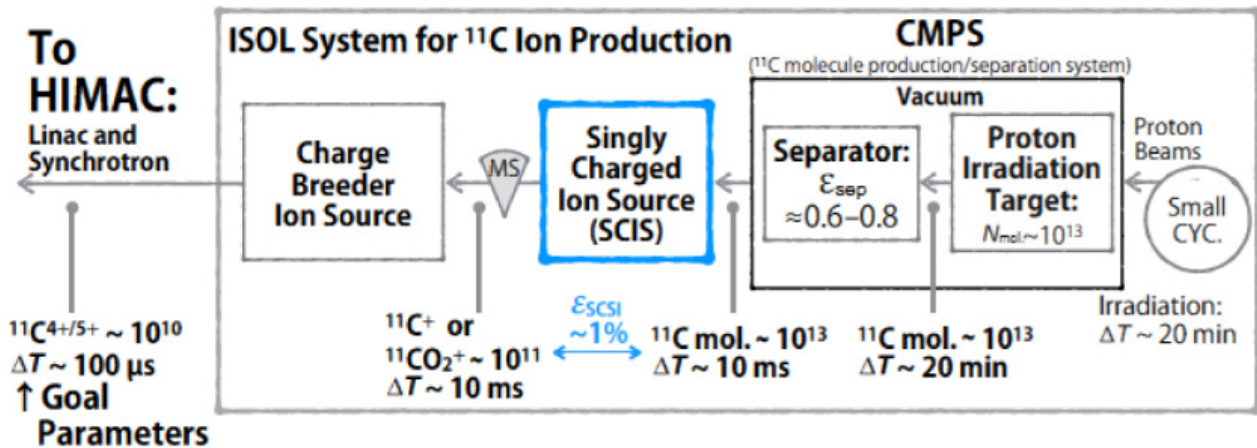
Figure 2: Sketch of the unstable ^{11}\text{C}^{4+} ion beam production for re-acceleration at HIMAC.
