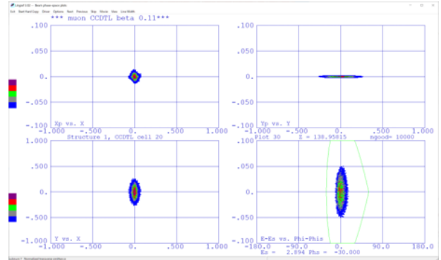
Figure 7: Phase distributions at the CCDTL exit with PARMILA.
