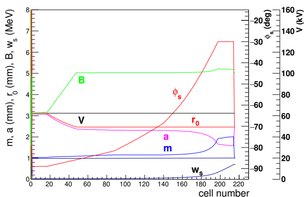
Figure 2: Cell Parameters of the L-band RFQ.
