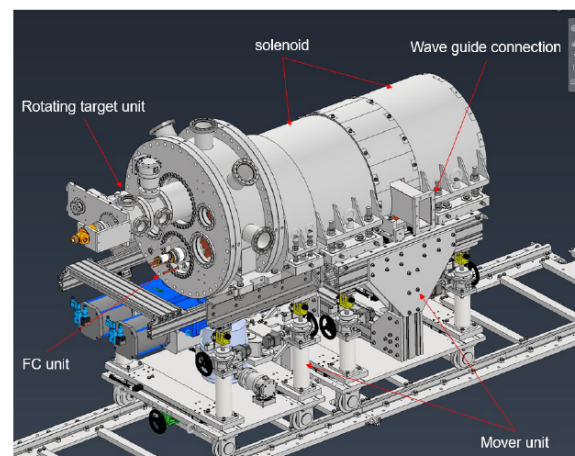
Figure 1: 3D model of the prototype positron source in the testbench.
