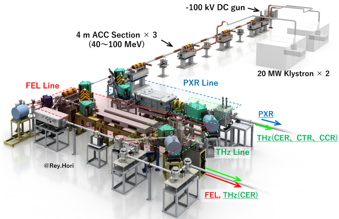
Figure 1: Layout of the 100 MeV electron linac, PXR line, FEL line, and THz line at LEBRA in Nihon University.
