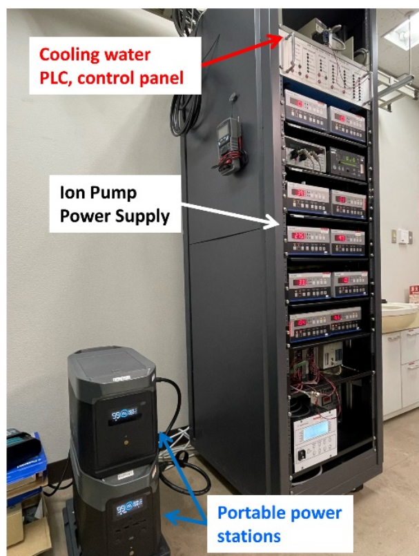
Figure 2: Portable power systems, ion-pump power supply and coolingwater control system rack.
