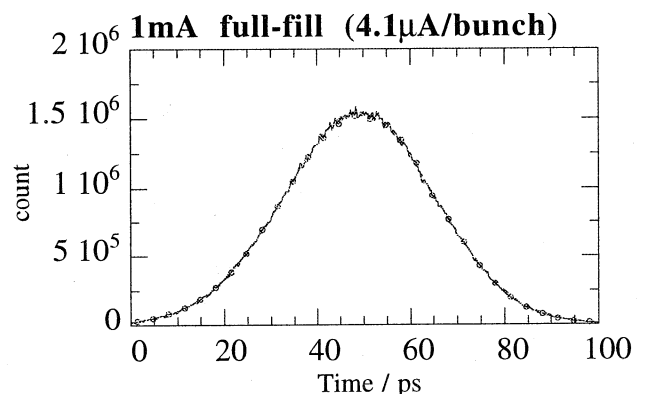
Fig. 2 bunch shape at low current. The solid line is a fitted curve using Gaussian shape with rms. = 16.3ps. The RF voltage is 11.6MV and the synchrotron frequency is 1520Hz. The calculated value from the natural energy spread is 16.6ps.
