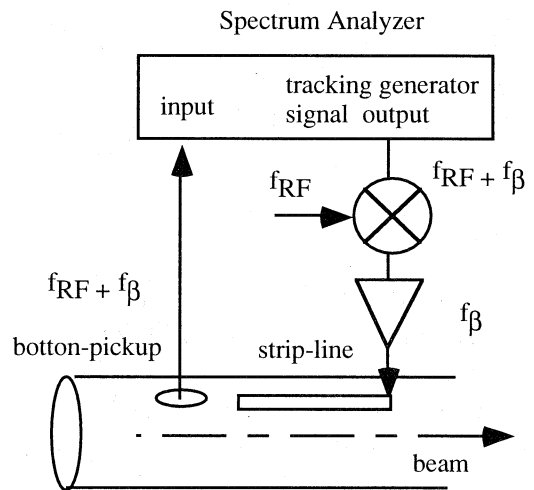
Fig. 5 Set-up for the measurement of the frequency response of the vertical betatron motion of the beam.
