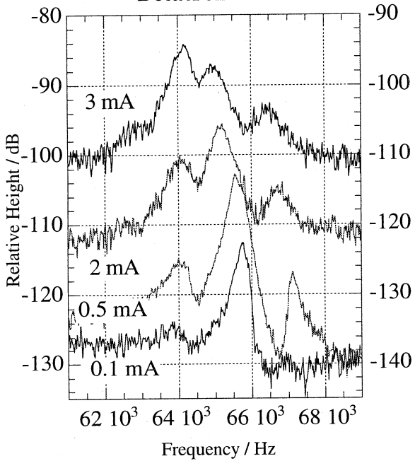
Fig. 6 Frequency response of vertical betatron motion vs. bunch current.
