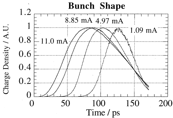
Fig. 3 Bunch shape and forward shift of bunch position. As the bunch current increases, the bunch has longer tail and the timing of bunch become earlier to compensate the parasitic energy loss of the bunch. The parasitic loss is the energy radiated to wake fields at impedance.
