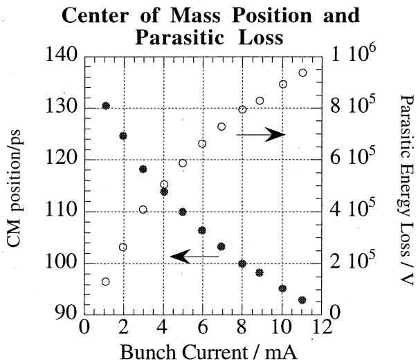
Fig. 4 Centre of Mass position of the bunch and calculated parasitic energy loss vs. bunch current.
