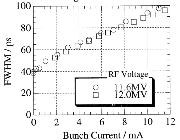
Fig. 1 Bunch length vs. bunch current at two values of the RF acceleration voltages.
