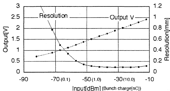
Figure 2: Output voltage and resolution for the SPBPM to the input signal power
