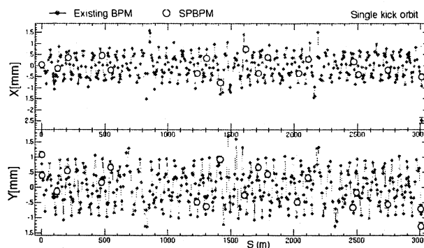
Figure 7: The consistency of the position sensitivity between the existing BPM and the SPBPM.
