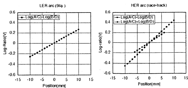
Figure 4: Log ratio value to the beam position on an axis of coordinates of LER BPM and HER BPM.
