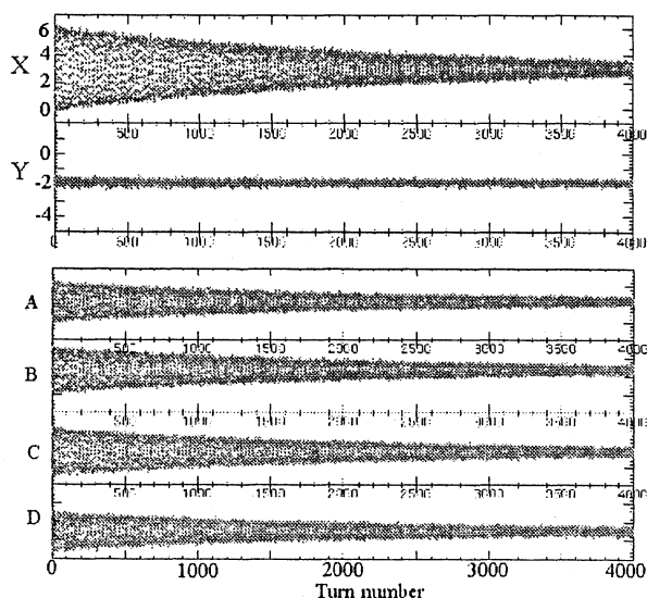
Figure 6: Beam position of turn by turn. Upper, Horizontal beam position; Middle, Vertical beam position; Lower, Four outputs of SPBPM.
