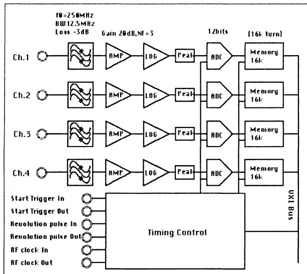
Figure 1: Block diagram for SPBPM
