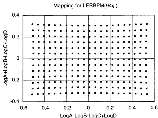
Figure 3: Mapping for the SPBPM
