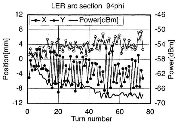
Figure 5: Orbital measurement of first injection of the positron beam to LER.
