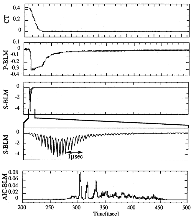
Figure 1: Current transformer and loss monitor signals of the KEK booster extraction. In this study, extraction bump magnet was excited to scatter beam particles. In CT signal, the delay time of 15 \mu\text{sec} is corrected
