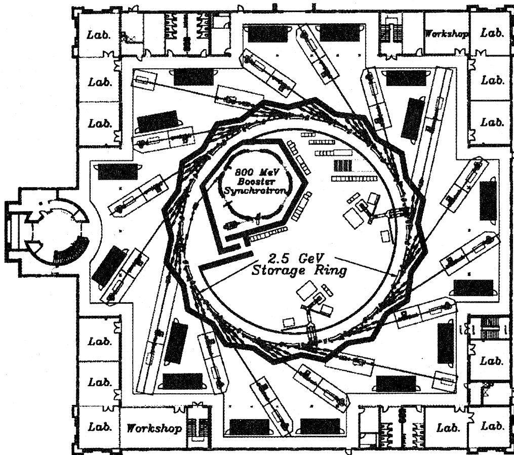
Figure 3: The layout of the accelerators
