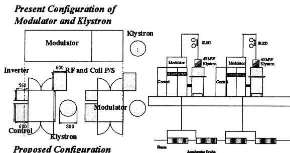
Figure 3 Comparison between the old and new modulator (left) and RF feeding scheme (right)
