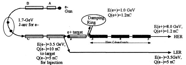
Figure 1 Proposed scheme using C-band system
