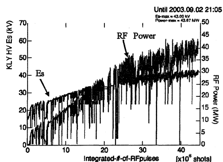
Figure 8 Processing history of accelerator guide with a function of shot numbers of rf pulse.
