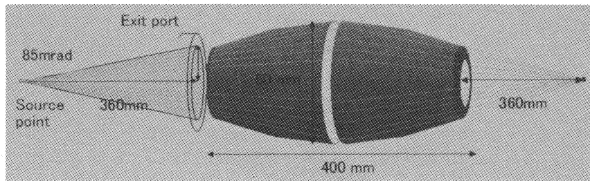
FIGURE 4: Eight sets of multi-layer cylindrical mirrors will be made by the replica method. Mother body must have the surface roughness less than nm and the shape tolerance less than 1 \mu m.
