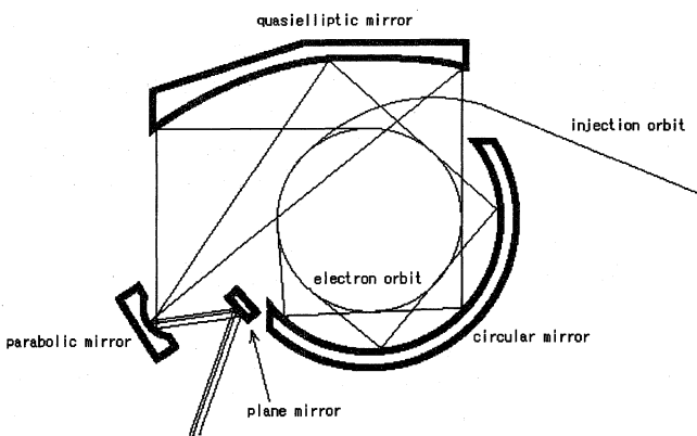
FIGURE 3: The special mirror system is composed of the circular mirror concentric to the electron orbit, quasi-elliptic mirror, which focuses the radiation in to one point,
