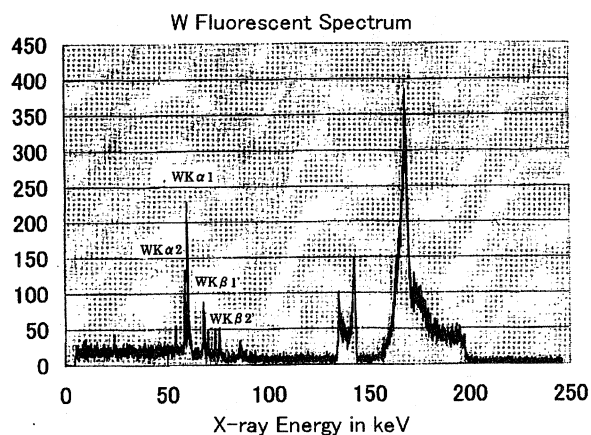
FIGURE 5: MIRRORCLE provides x-ray fluorescent analysis of heavy elements, while it is possible with more than 5 GeV SR sources.
